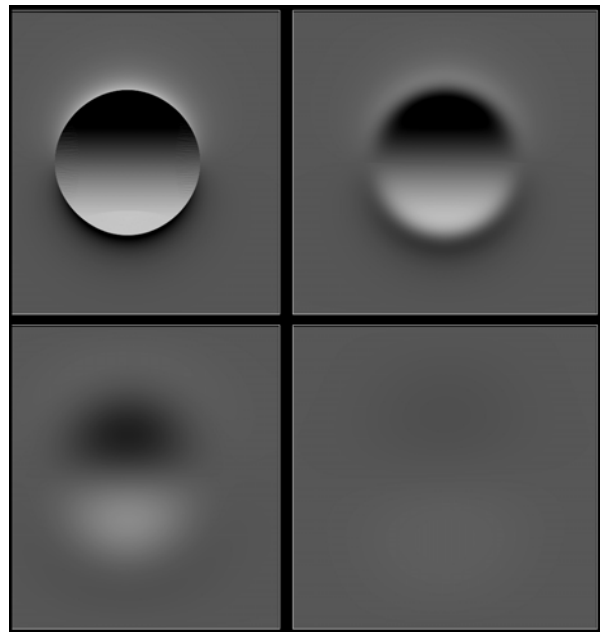
Figure 2: A demonstration of the downslope motion module, showing gradual crater degradation due to impact-induced seismic shaking.
